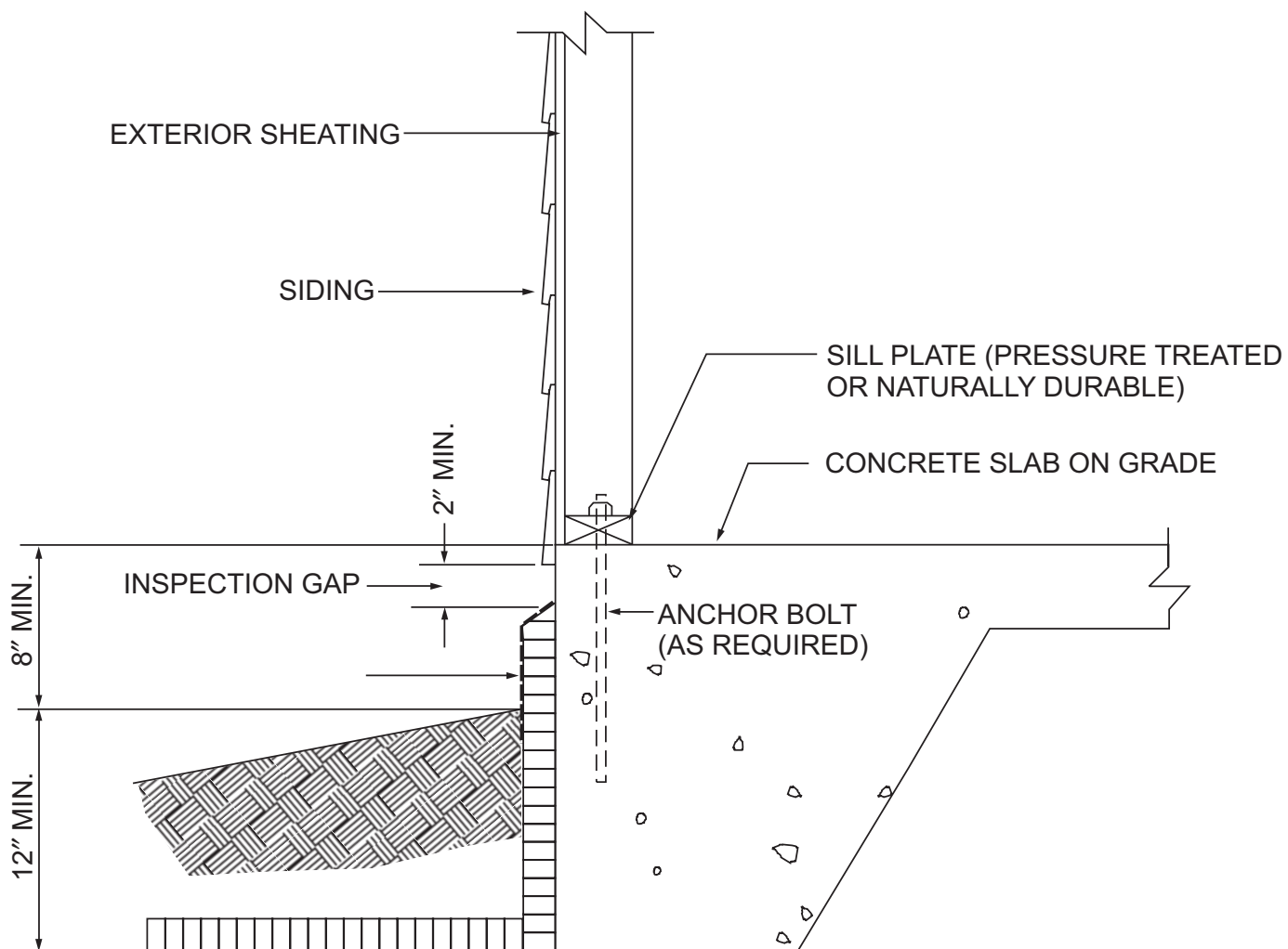
FOUNDATION INSULATION 24" VERTICAL DEPTH OR A COMBINATION OF VERTICAL AND HORIZONTAL DIMENSION EQUAL TO 24"
